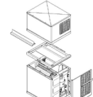
STACKING KIT
