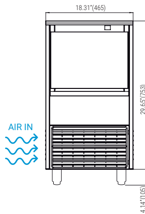
FRONTAL VIEW
