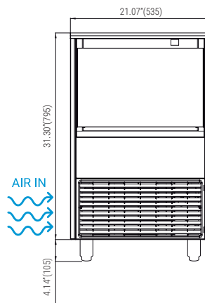
FRONTAL VIEW
